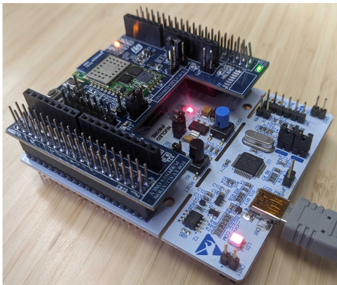
Fig. 5: The STM32-NucleoF401RE board (expanded with an X-NUCLEO-IDW01M1 Wi-Fi Module) used in our experiments.
